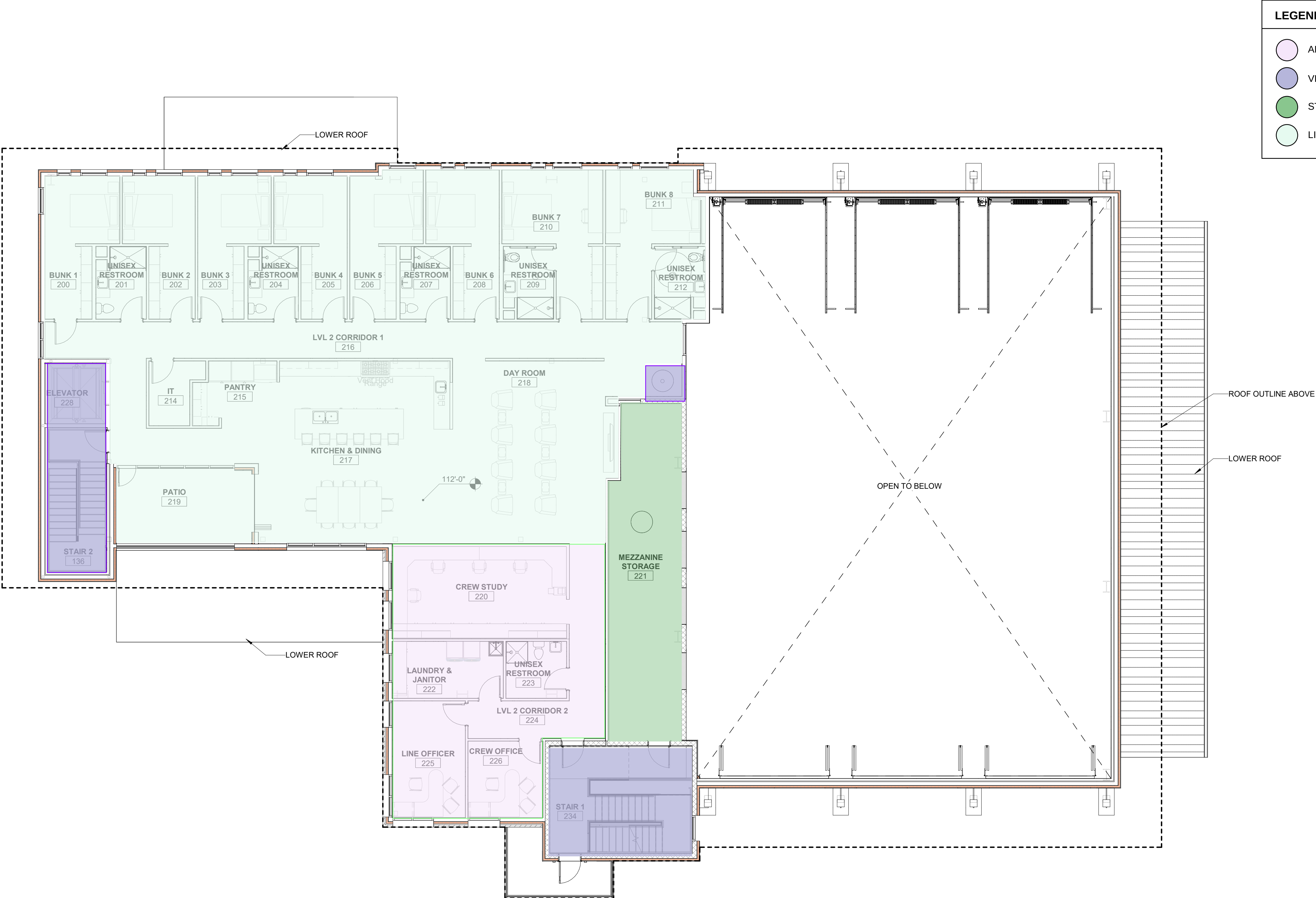
1 FLOOR PLAN - LEVEL 2 OVERALL 1/8" = 1'-0"
